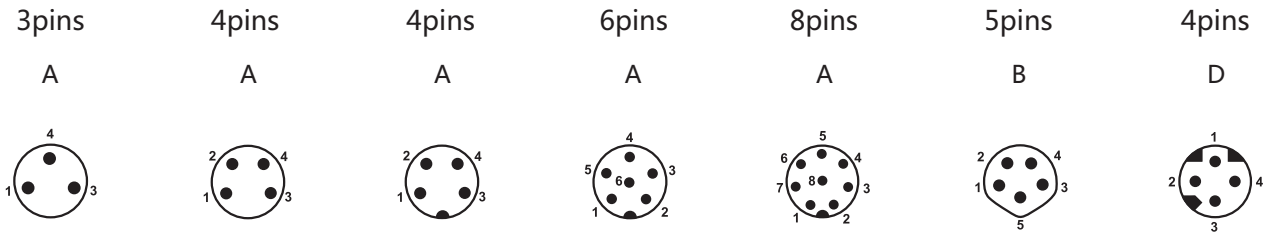
Contact layout/针孔排布 (Front view/前视图)
