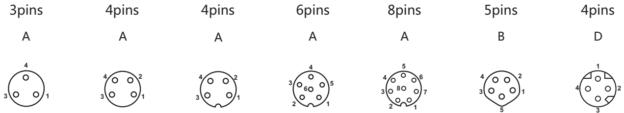
Contact layout/针孔排布 (Front view/前视图)
